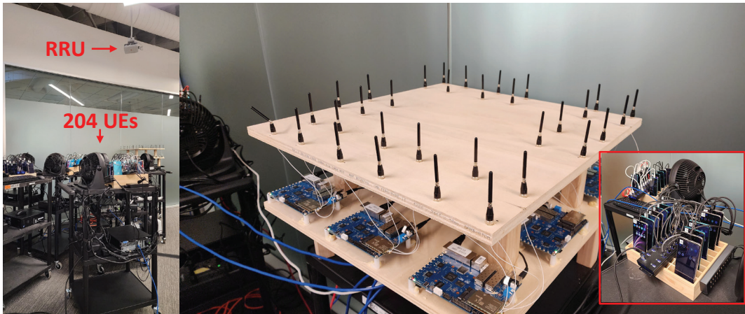
Figure 2. UE Placement
