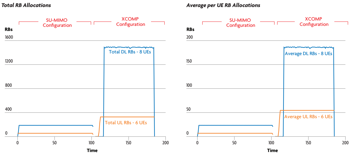
Figure 6. Downlink and Uplink Resource Block Allocations with 8 Distributed UEs – SU-MIMO and XCOMP Configurations
