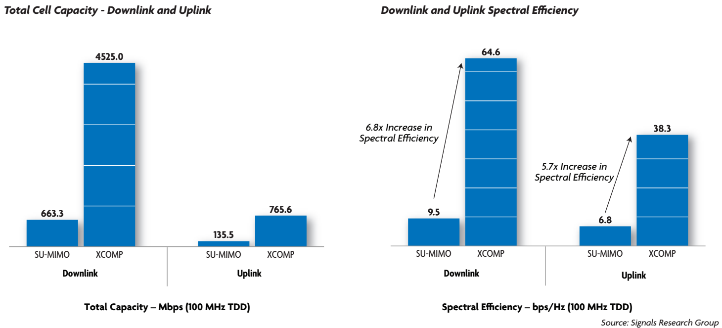
Figure 5. Bidirectional Capacity and Spectral Efficiency with 8 Distributed UEs – SU-MIMO and XCOMP Configurations
